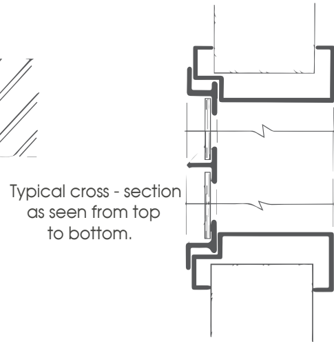
Typical cross-section viewed from the top.
