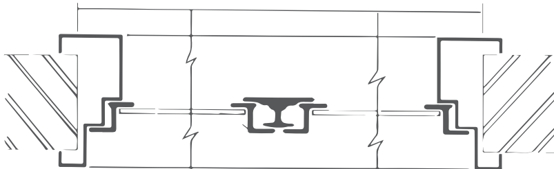
Typical cross-section viewed from the top.
