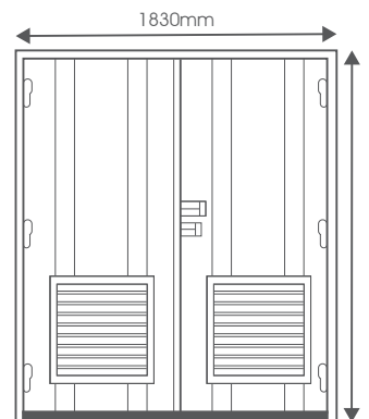
Double Door Type G No Louvre Panel Type GV Bottom Louvre Panel Type GVV Top & Bottom Louvre Panels Type GVA Full Louvre Vents
