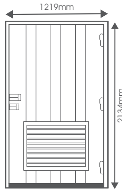
Single Door Type C No Louvre Panel Type CV Bottom Louvre Panel Type CW Top & Bottom Louvre Panels Type CVA Full Louvre Vents
